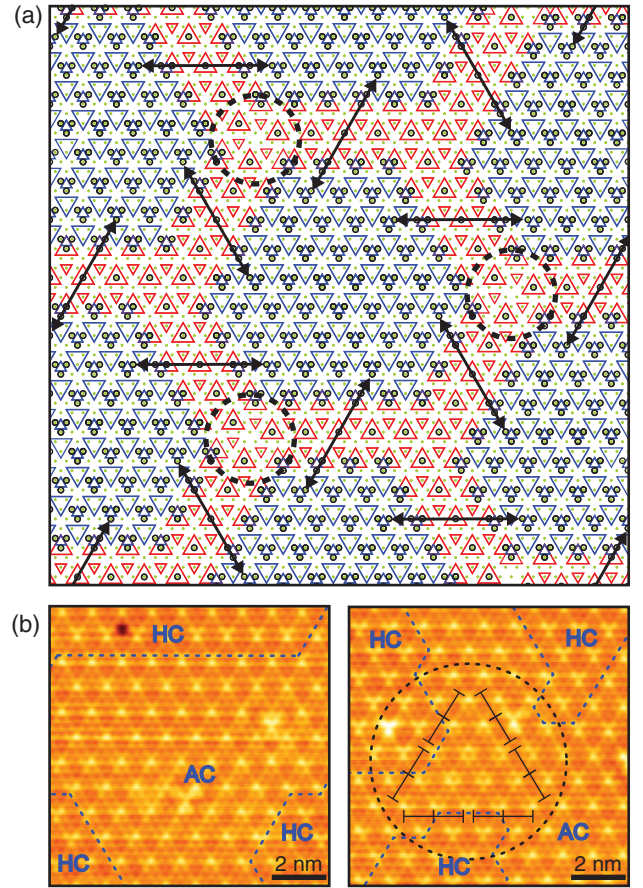
FIG. 4. (a) Atomistic schematics of an ideal honeycomb structure of the HC CDW domains and discommensurations which are composed of type I and II vertices. The black dashed circle denotes the region of AC CDW dislocation and the black arrows the directions of CDW translations among the HC CDW domains. (b) STM topography of type I (left) and II (right) vertices where three AC CDW stripe domains merge. Black dashed circle indicates the region of AC CDW dislocations. Black solid lines represent the dislocations among the AC structures.
