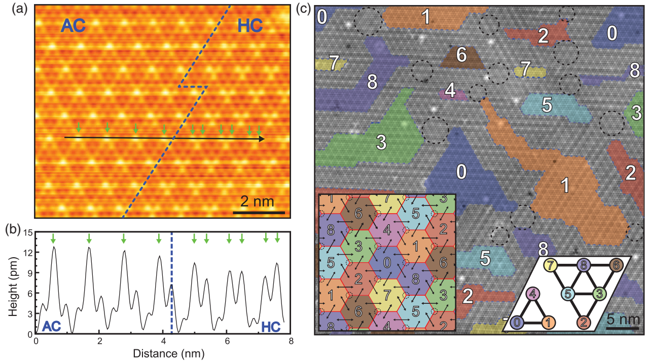
FIG. 1. (a) STM topography of the coexisting domains in 2H-NbSe 2 at a sample bias of 100 mV. The blue dashed line separates two different domains. (b) Line profile along the black arrow in (a). Green arrows indicate the locations of bright topographic protrusions. (c) STM topography of HC CDW domains at 100 mV. Black dashed circles indicate the region of AC CDW dislocations as magnified in Fig. 4(b). The colors and numbers indicate particular HC CDW domains among nine translationally degenerate domains. These domains have to be connected properly in the ideal domain network shown in the insets. Different domains are identified by their relative translation as defined in the right inset within one CDW unit cell. The black arrows represent the directions of CDW translations among HC CDW domains.
